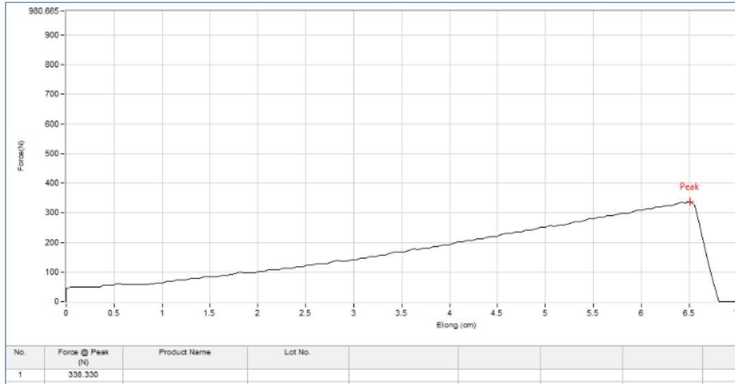
Tensile Graph Before UV Test
